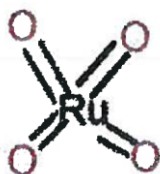
(ruthenium(VIII)oxide)
